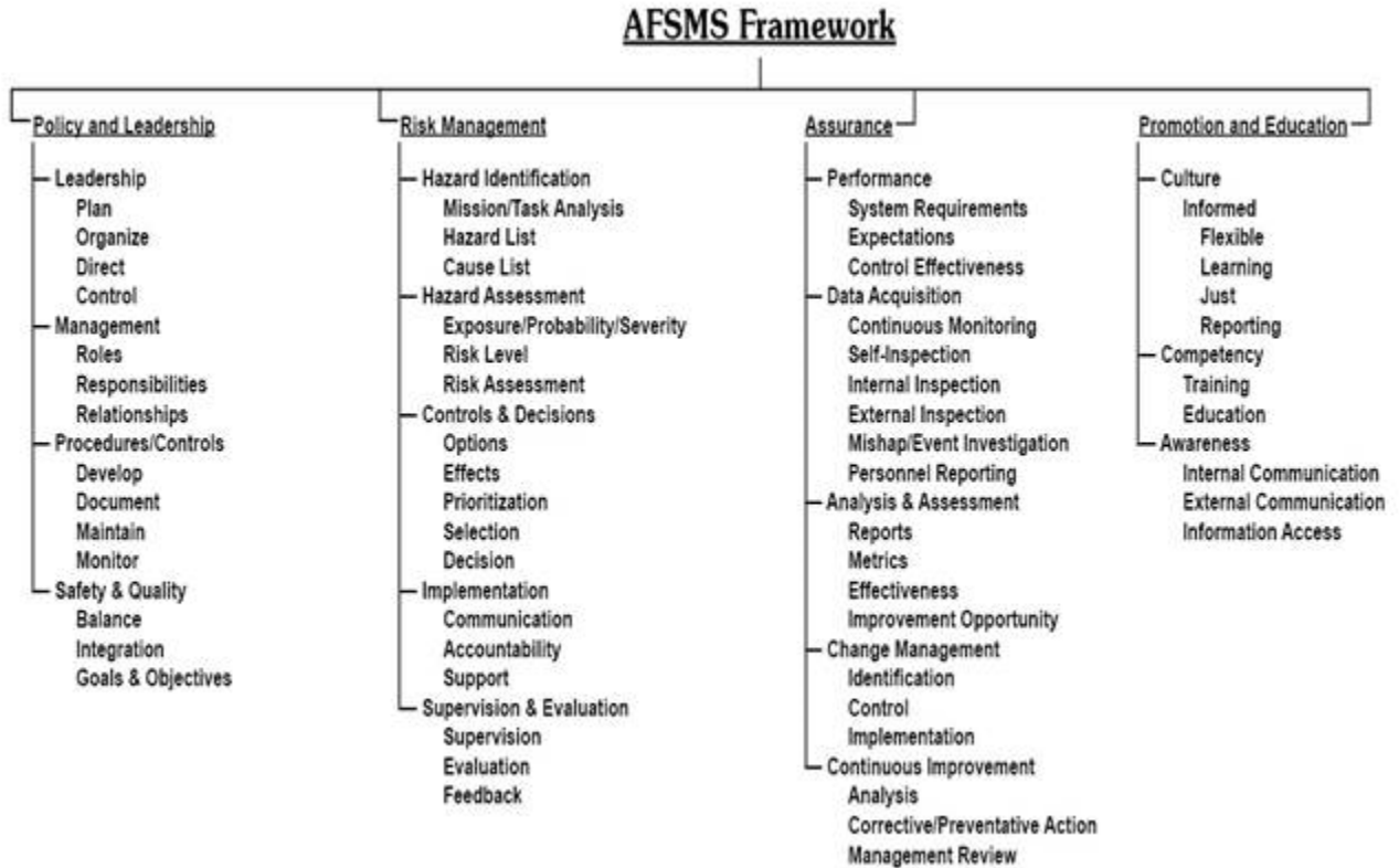
Figure 13.2. AFSMS Framework.
